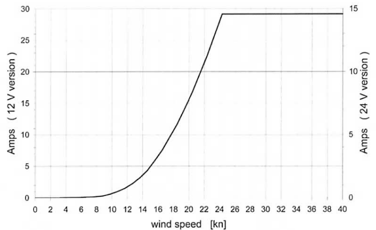
Charging Current
