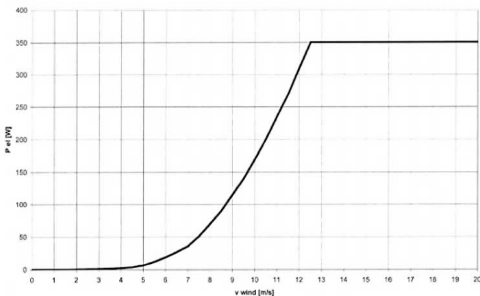
Power Curve
